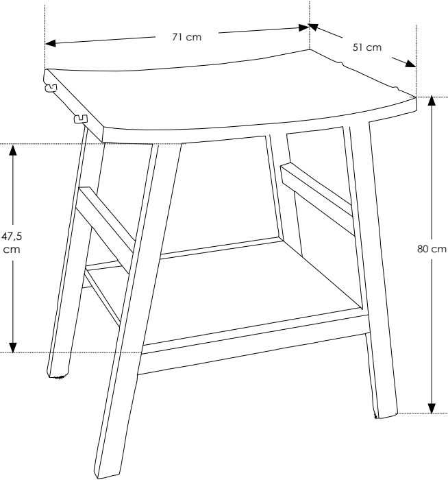
CP880 ZXL Misure - Sizes 51 x 71 x 80 cm
