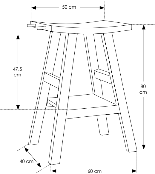
CP880/Z CONSOLLE Misure - Sizes 40 x 60 x 80 cm
