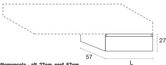
Cassetto sottomensola - alt. 27cm, prof. 57cm Undershelf drawer - height 27cm, depth 57cm
