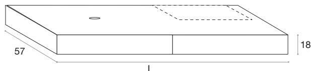
Mensola portalavabo con cassetti - alt. 18cm, prof. 57cm Washbasin stand shelf with drawers - height 18cm, depth 57cm
