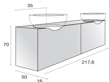
Scarico a centro stanza - versione free-standing Siphon on the floor - free standing version
