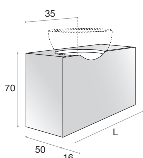
Scarico a centro stanza - versione free-standing Siphon on the floor - free standing version
