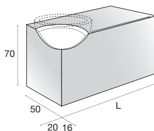
Scarico a centro stanza - versione free-standing Siphon on the floor - free standing version
