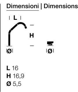
Comando remoto in Corian con canna orientabile in acciaio Aisi 316l Mixer group with remote control on deck and swivel spout made in stainless steel Aisi 316l
