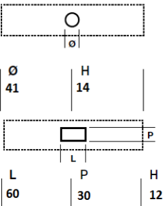
Dimensioni lavabo | Washbasin dimensions
