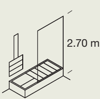
Unico semincasso | semi recessed (Corian) L 170-180-190 P 80-90 H 45-25
