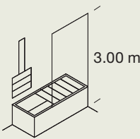
Unico (Corian) L 170-180-190 P 80-90 H 55
