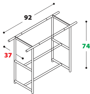
Console L92 x H74 x P35 Console L92 x H74 x P35
