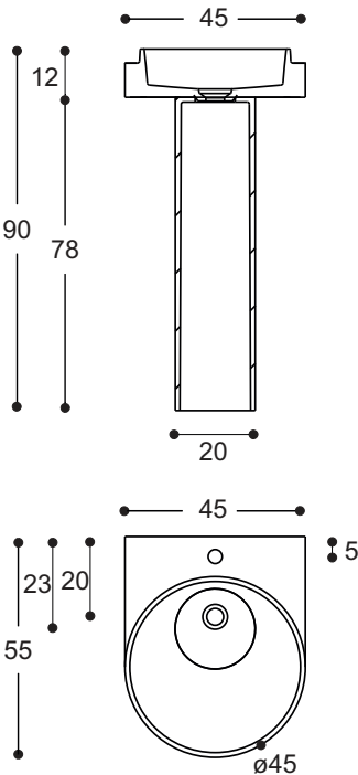
wash-basin in Pietra vasque en Pierre
