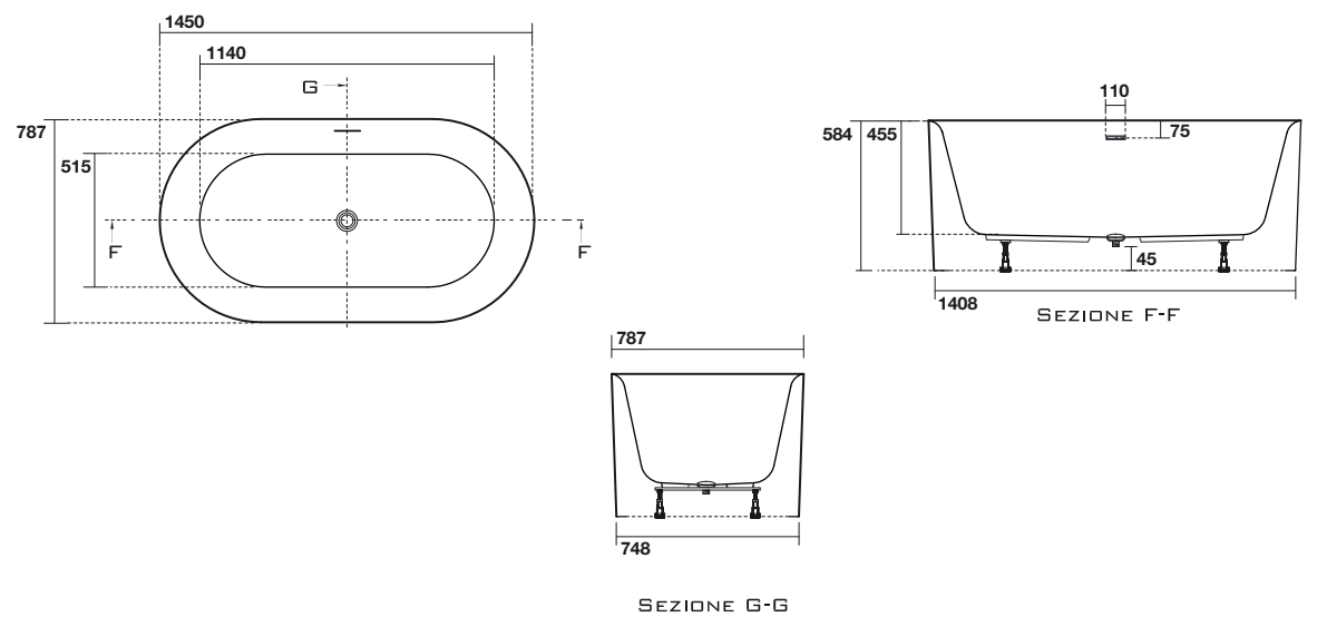
5350 Vasca freestanding NoLIta 145x78xh58 in acrilico, completa di piletta clic-clac NoLIta freestanding acrylic bath tub with push down drain plug
