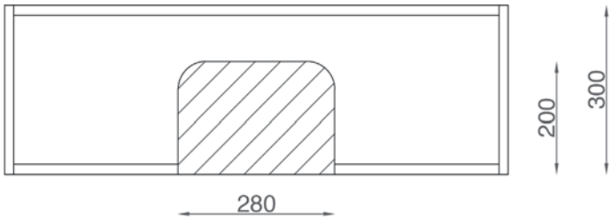
LIGNUM H.40 VANO SCARICHI- SPACE FOR WASTE OUTLET
