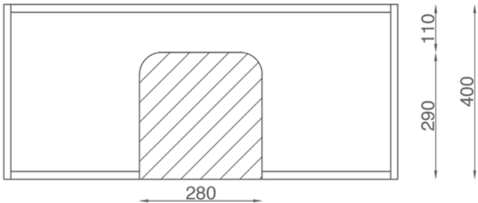
LIGNUM H.60 VANO SCARICHI- SPACE FOR WASTE OUTLET
