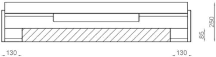
KS H.45 CM VANO SCARICHI - SPACE FOR WASTE OUTLET
