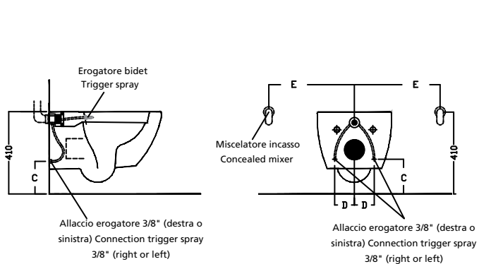
Vaso Sospeso-Wall-hung WC-Hang Wc
