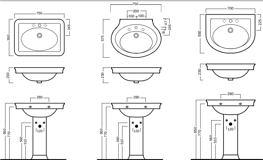
Y0EK01 colonna pedestal
