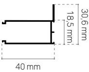
profilo murale profilé mural_wall profile
