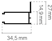
profilo compensatore e murale profilé de compensation et mural_adjustability and wall profile
