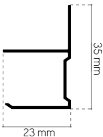
profilo murale profilé mural_wall profile
