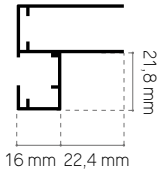
profilo compensatore e murale profilé de compensation et mural_adjustability and wall profile
