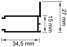
profilo murale profilé mural_wall profile
