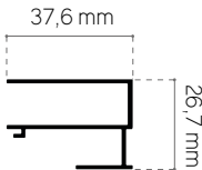
profilo murale profilé mural / wall profile
