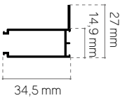
profilo compensatore e murale profilé de compensation et mural_adjustability and wall profile
