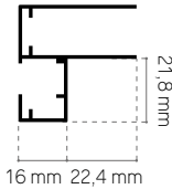
profilo compensatore e murale profilé de compensation et mural_adjustability and wall profile
