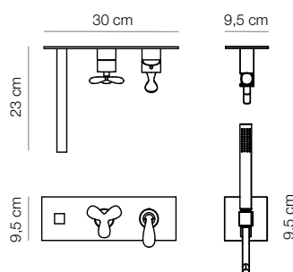
WALL-MOUNTED SINGLE-LEVER MIXER FOR BATHTUB, OUTLET, SHOWER HEAD AND MIXER
