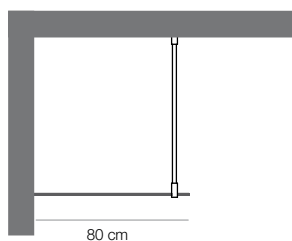
CORNER INSTALLATION
