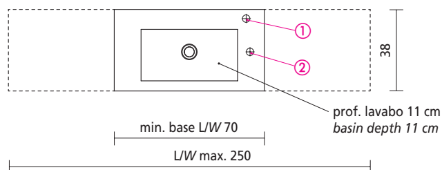
VASCA SINGOLA LAVABO BOTTE 500 (RPM) / SINGLE-BOWL BOTTE 500 (RPM) BASIN Misure interne / Interior dimensions L/W 46 x P/D 27 x H 11 cm
