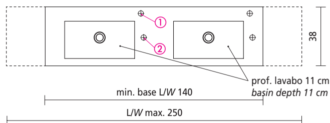
VASCA DOPPIA LAVABO BOTTE 500 (RPM) / DOUBLE-BOWL BOTTE 500 (RPM) BASIN Misure interne / Interior dimensions L/W 46 x P/D 27 x H 11 cm
