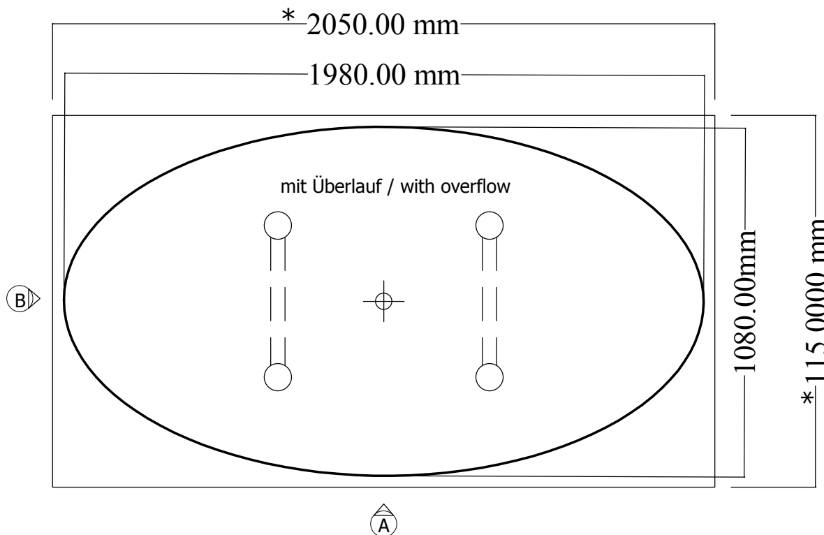
Grundriss / plan view
