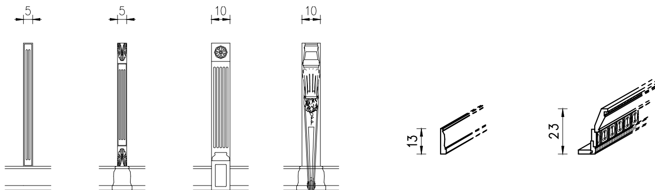
Ante, cassetti, colonne decorative, zoccolo e cimasa / Doors, drawers, decorative pillars and frames
