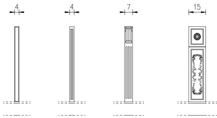
Ante, cassetti, colonne decorative, zoccolo e cimasa / Doors, drawers, decorative pillars and frames
