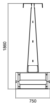
Cavalletto in lamiera zincata Zinc-plated sheet A-frame
