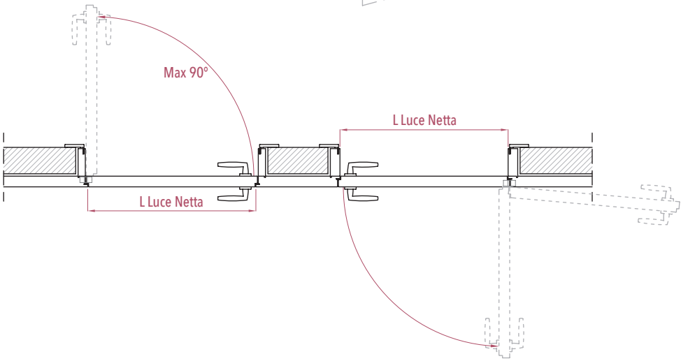
INFINITY - PORTA A SPINGERE
