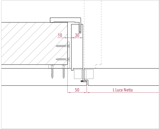
INFINITY - PORTA A SPINGERE
